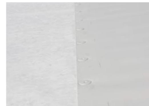
Fully fastened roofing membrane. Marks are pre-printed onto the membranes to ensure a proper overlapping of the next sheet.
