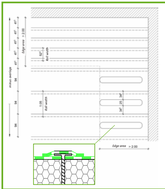
Example Fastening Plan
